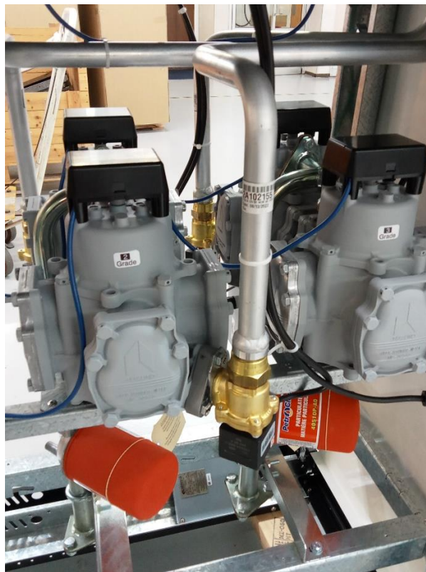
Tatsuno Model MP-02515 meters
