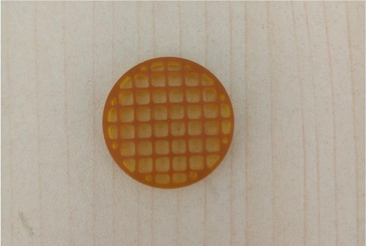
Flow conditioner
