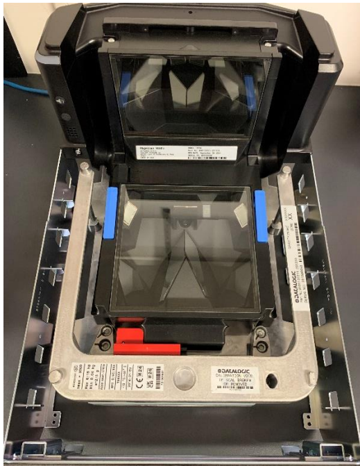
(b) Datalogic Model Magellan 9556 Weighing Instrument With Load Receptor Plate Removed (Pattern)
