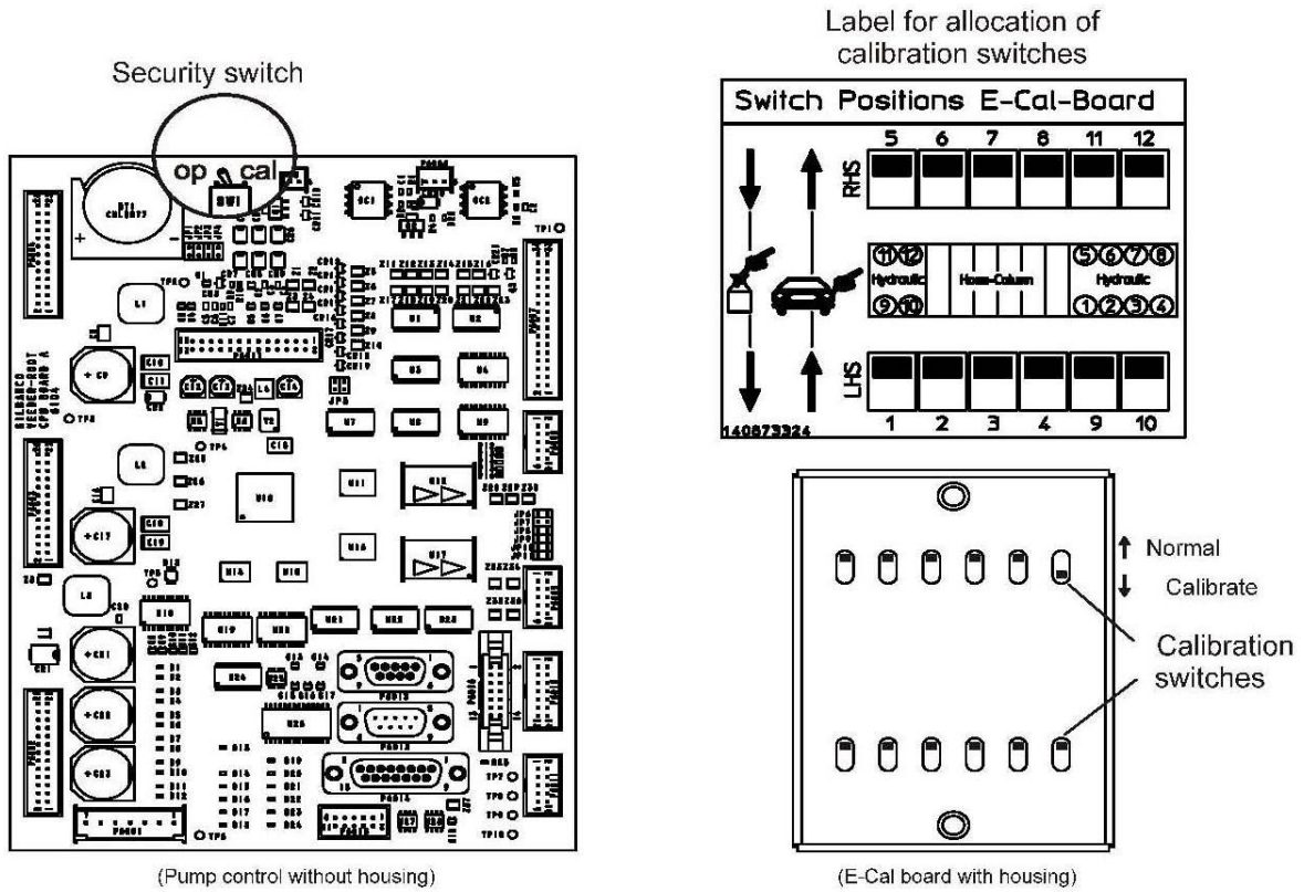
(a) Electronics Sealing – Sealing of Petrol/Diesel/LPG Meter Calibration Access (destructible adhesive labels used for security and calibration switches)
