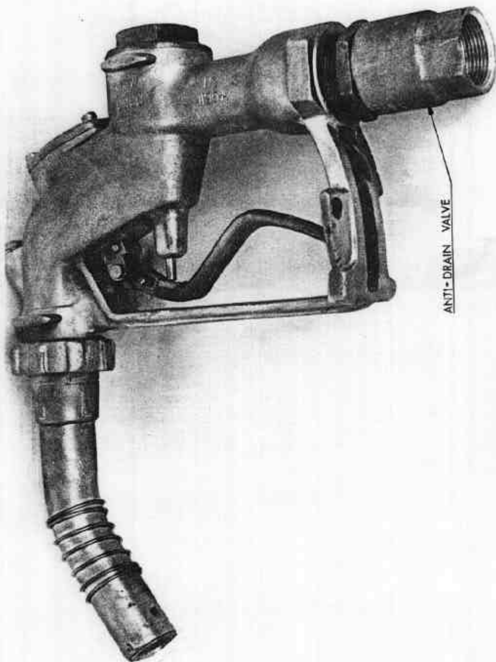
OPW 1190AS Automatic Hose Nozzle with External Anti-drain Valve
