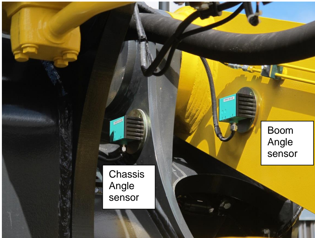
Boom and Chassis Inclinometers
