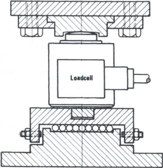
More Alternative Mounting Arrangements
