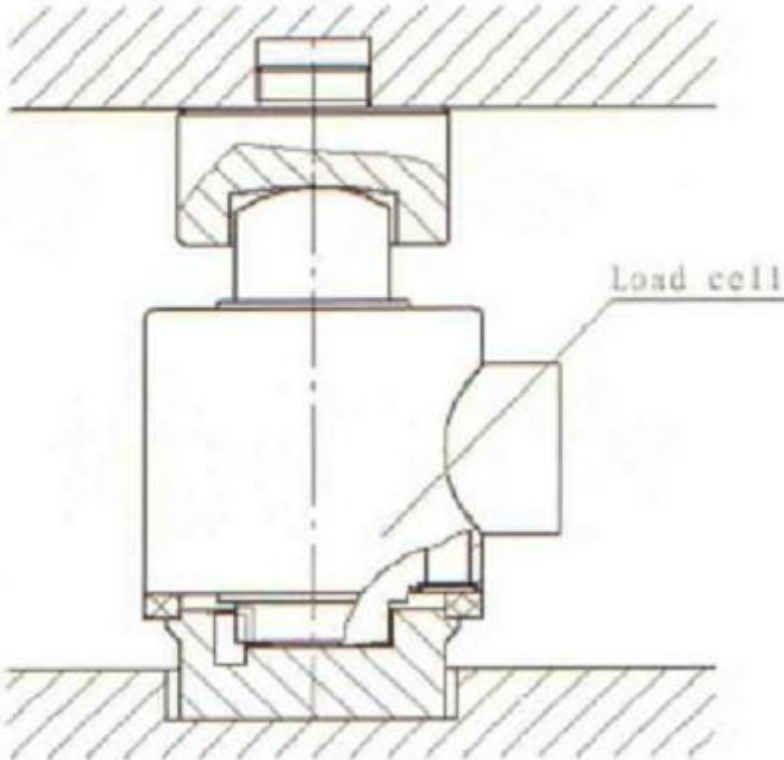
A Typical Mounting Arrangement
