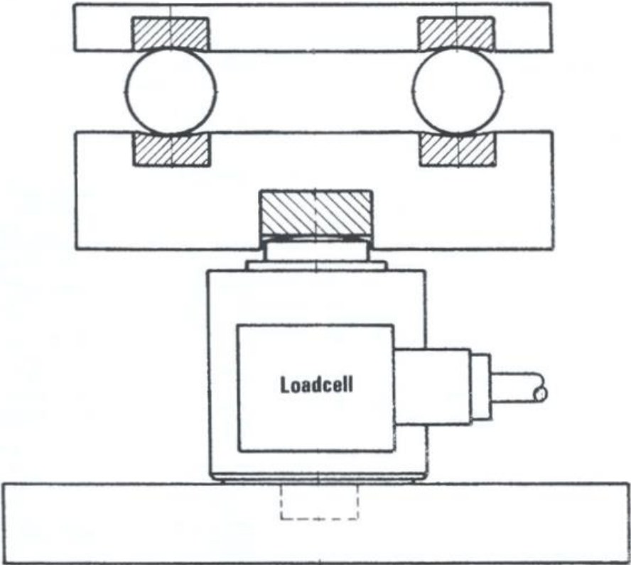
Some Alternative Mounting Arrangements
