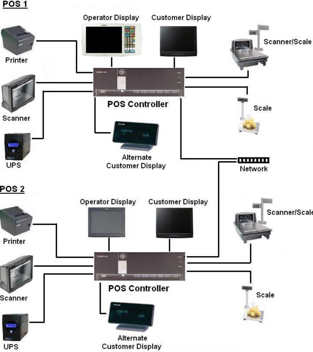
Worldsmart Model WinPOS Point of Sale (POS) System
